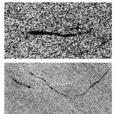
Examples of a potential seepage slicks offshore Labrador
